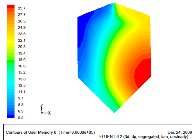
Figure 2. The distribution of phosphine concentration (mg/litre) on a diametrical plane in a circular silo containing cotton seed after 100 hours of operation. The phosphine is introduced into the silo through a small hole on the lower right of the plane whence it disperses non-uniformly through the grain, the effect of which is exacerbated by the sorption on and reaction by of the fumigant on the grain.
