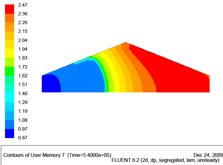
Figure 1. The ratio of potential population increase of R. dominica in wheat that has an initial moisture content of 12% (wet basis) and temperature of 35°C, after having been aerated for 150 hours with air that has a temperature of 10°C and a humidity of 0.007 kg water/kg dry air. The specific flow rate of the air is 2 litres per second per tonne of grain.
