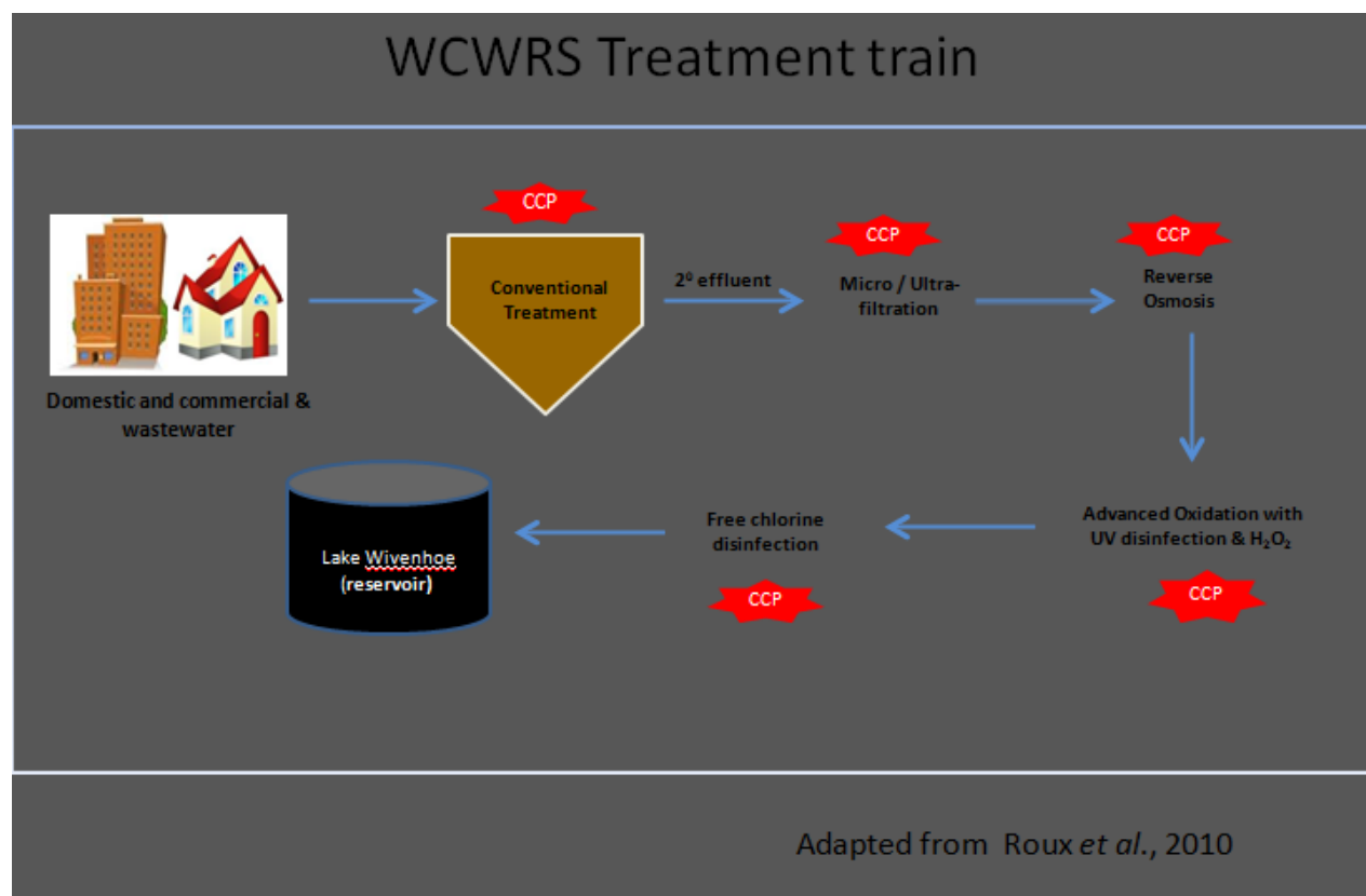
Figure 2: Western Corridor Recycled Water Scheme treatment train.
