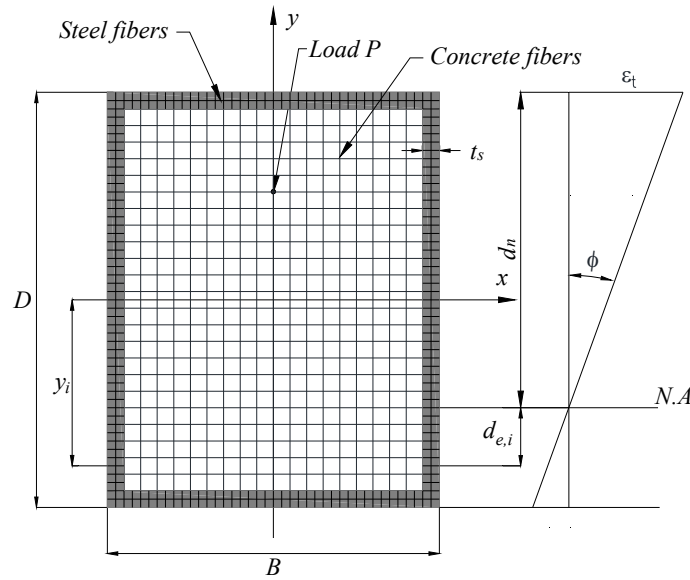
Fig. 1. Typical fiber mesh and strain distribution in the cross-section of a rectangular CFST column under uniaxial bending.
