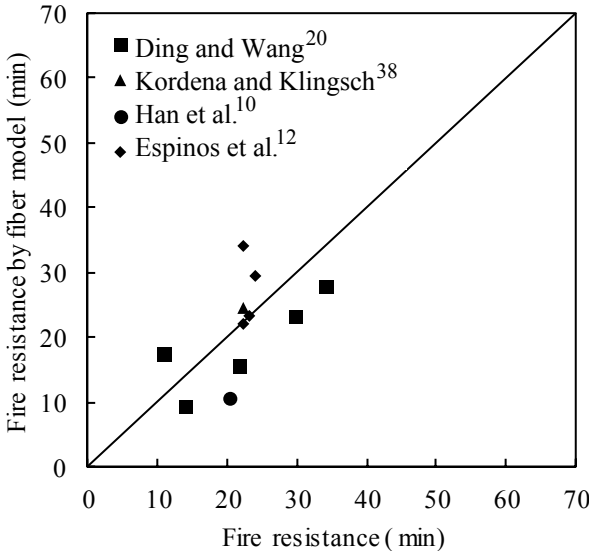
Fig. 5. Comparison of fire-resistance times predicted by the present fiber model with those obtained from testes and finite element analyses.
