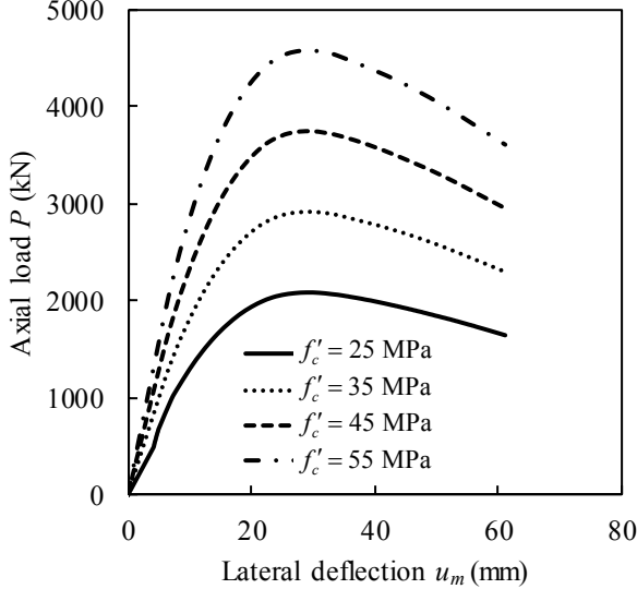
Fig. 12. Effects of concrete strength on the structural responses of rectangular slender CFST columns at the fire exposure time of 40 min.
