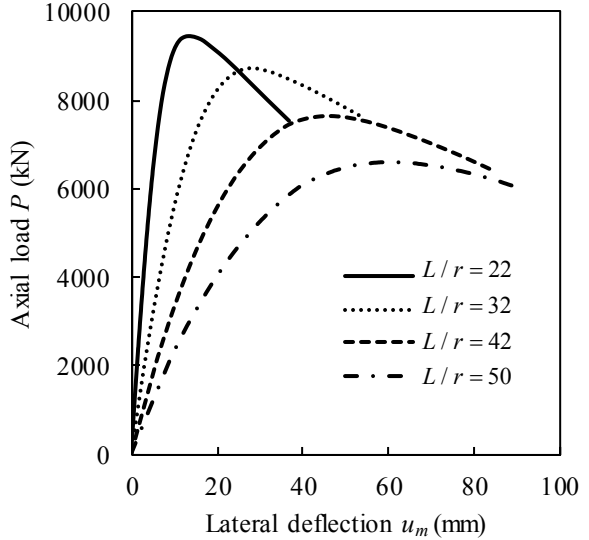
Fig. 8. Effects of column slenderness on the axial load-deflection responses of square CFST columns at the fire exposure time of 40 min.
