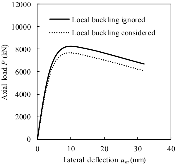
Fig. 6. Influences of local buckling on the axial load-deflection responses of slender square CFST column at the fire exposure time of 20 min.
