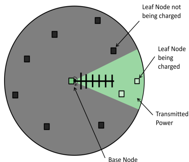
Figure 1. The RF transfer system setup.
