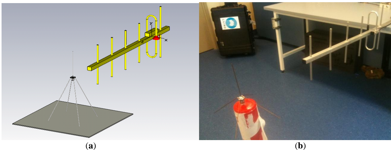
Figure 5. (a) The Microwave Studio model of the Yagi antenna and the whip antenna separated by 90 cm; (b) simulation verification in the laboratory.
