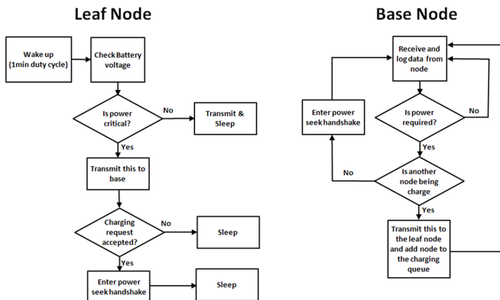
Figure 4. The programming process flow diagrams used for the leaf and base node.
