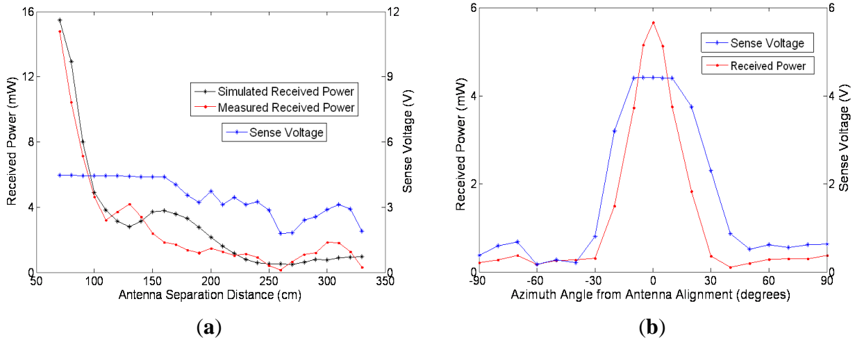
Figure 6. (a) Received power and sense voltage as separation distance increases; (b) Plot of received power and sense voltage at different azimuth angles for antennas at 1-meter separation.
