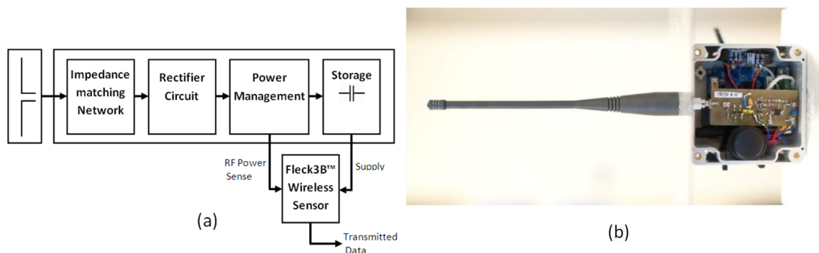
Figure 2. The leaf node: (a) harvesting circuit block diagram and (b) showing the power receiving antenna, harvesting circuit and Fleck TM 3B sensor.
