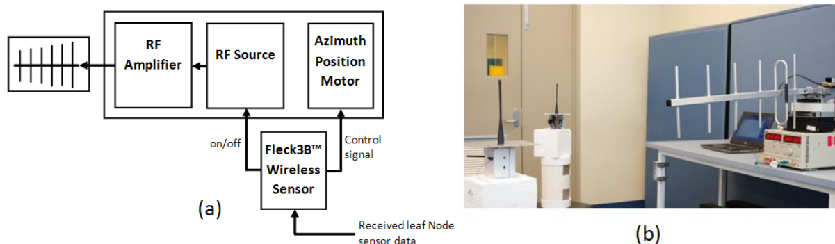
Figure 3. The base node: (a) power transmitter circuit and (b) the experimental setup showing the base node, the transmitting antenna, the rotator, and two leaf nodes.
