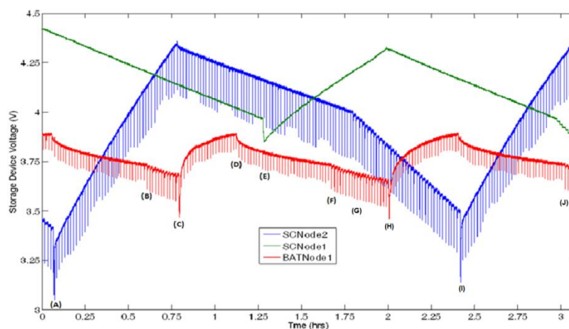
Figure 8. Storage voltage of three nodes being powered from the system.
