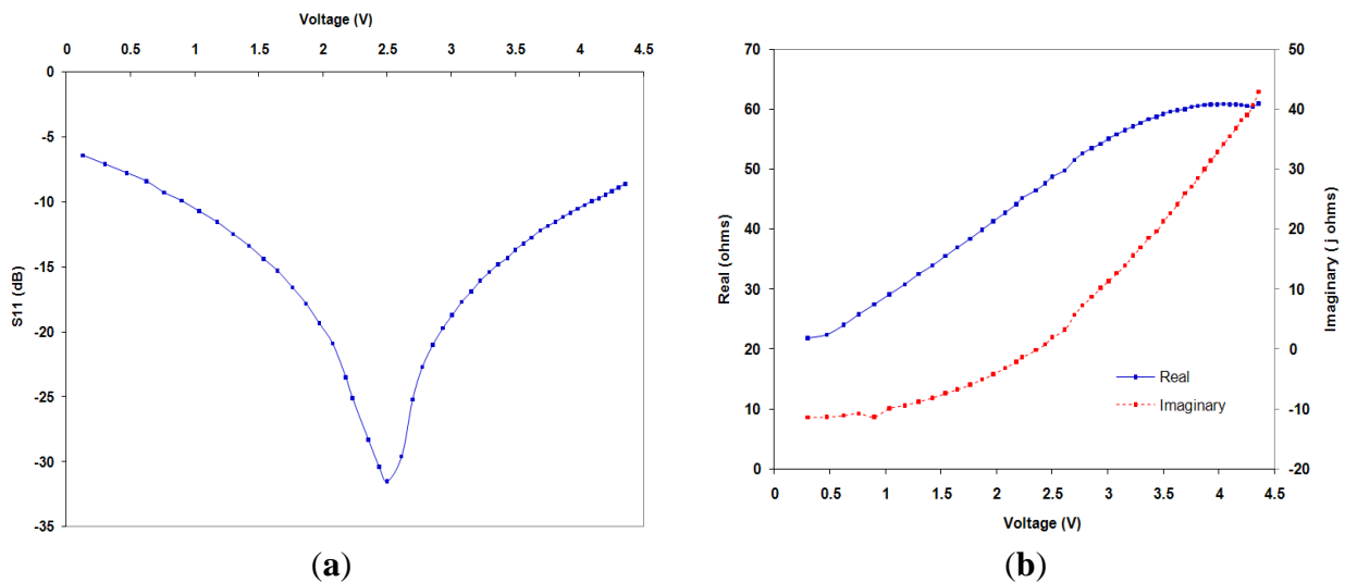
Figure 7. (a) change of S11 as supercapacitor charges at 6 dBm; (b) Impedance change as supercapacitor charges.
