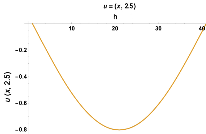
Figure 6. The relation between the numerical and exact solutions of the dispersive equation at h = 0.025, k = 0.0005, \alpha = \frac{h^3}{160}, \beta = -\alpha + \frac{h^3}{2}, t = 2.5 .
