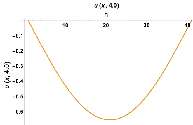
Figure 9. The relation between the numerical and exact solutions of the dispersive equation at h = 0.025, k = 0.0005, \alpha = \frac{h^3}{160}, \beta = -\alpha + \frac{h^3}{2}, t = 4.0 .
