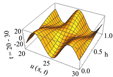
Figure 14. The 3D for the numerical solutions of the dispersive equation from t = 20 to t = 30 .
