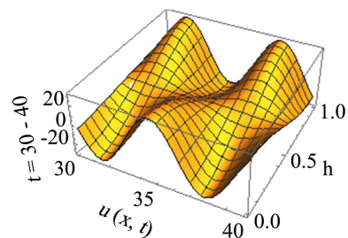
Figure 15. The 3D for the numerical solutions of the dispersive equation from t = 30 to t = 40 .
