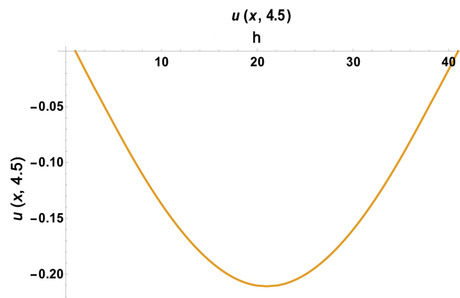
Figure 10. The relation between the numerical and exact solutions of the dispersive equation at h = 0.025, k = 0.0005, \alpha = \frac{h^3}{160}, \beta = -\alpha + \frac{h^3}{2}, t = 4.5 .
