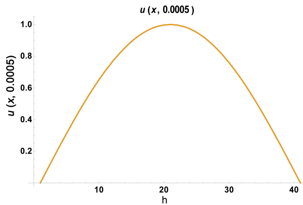
Figure 1. The relation between the numerical and exact solutions of the dispersive equation at h = 0.025, k = 0.0005, \alpha = \frac{h^3}{160}, \beta = -\alpha + \frac{h^3}{2}, t = 0.0005 .
