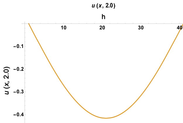
Figure 5. The relation between the numerical and exact solutions of the dispersive equation at h = 0.025, k = 0.0005, \alpha = \frac{h^3}{160}, \beta = -\alpha + \frac{h^3}{2}, t = 2.0 .
