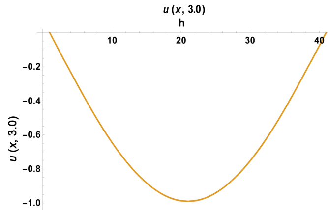
Figure 7. The relation between the numerical and exact solutions of the dispersive equation at h = 0.025, k = 0.0005, \alpha = \frac{h^3}{160}, \beta = -\alpha + \frac{h^3}{2}, t = 3.0 .
