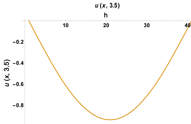
Figure 8. The relation between the numerical and exact solutions of the dispersive equation at h = 0.025, k = 0.0005, \alpha = \frac{h^3}{160}, \beta = -\alpha + \frac{h^3}{2}, t = 3.5 .
