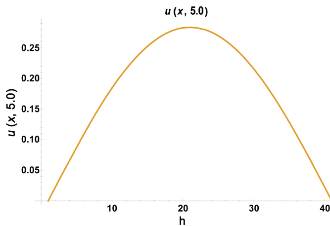
Figure 11. The relation between the numerical and exact solutions of the dispersive equation at h = 0.025, k = 0.0005, \alpha = \frac{h^3}{160}, \beta = -\alpha + \frac{h^3}{2}, t = 5.00 .
