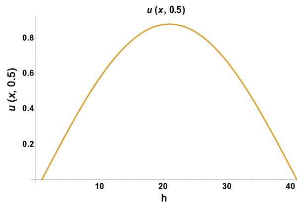
Figure 2. The relation between the numerical and exact solutions of the dispersive equation at h = 0.025, k = 0.0005, \alpha = \frac{h^3}{160}, \beta = -\alpha + \frac{h^3}{2}, t = 0.5 .
