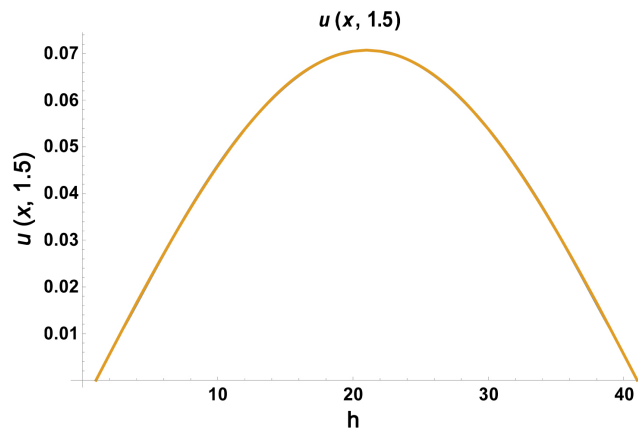
Figure 4. The relation between the numerical and exact solutions of the dispersive equation at h = 0.025, k = 0.0005, \alpha = \frac{h^3}{160}, \beta = -\alpha + \frac{h^3}{2}, t = 1.5 .
