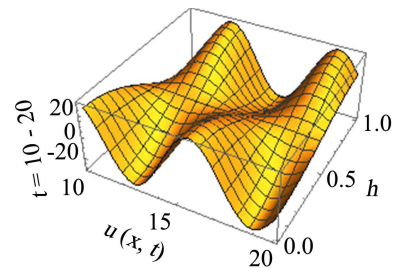
Figure 13. 3D for the numerical solutions of the dispersive equation from t = 10 to t = 20 .
