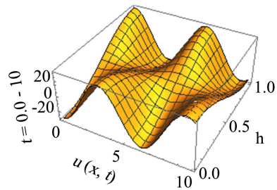
Figure 12. 3D for the numerical solutions of the dispersive equation from t = 0 to t = 10 .
