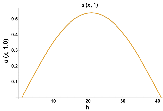
Figure 3. The relation between the numerical and exact solutions of the dispersive equation at h = 0.025, k = 0.0005, \alpha = \frac{h^3}{160}, \beta = -\alpha + \frac{h^3}{2}, t = 1.0 .
