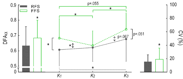
Figure 2. Group mean and SD of DFA \alpha values averaged across shoe types for each group, and over the three task-relevant sub-phases of the stance phase. Bar graphs show between-group (FFS vs RFS) differences for average DFA \alpha and average CV across sub-phases and shoe type. *Represents significance level p < 0.05 ; for group \times phase interaction effects, and pairwise comparisons for between group and between phase.
