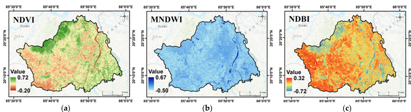
Figure 3. Landscape indices for Bhubaneswar: (a) Normalised Difference Vegetation Index (NDVI); (b) Modified Normalised Difference Water Index (MNDWI); and (c) Normalised Difference Built-up Index (NDBI).
