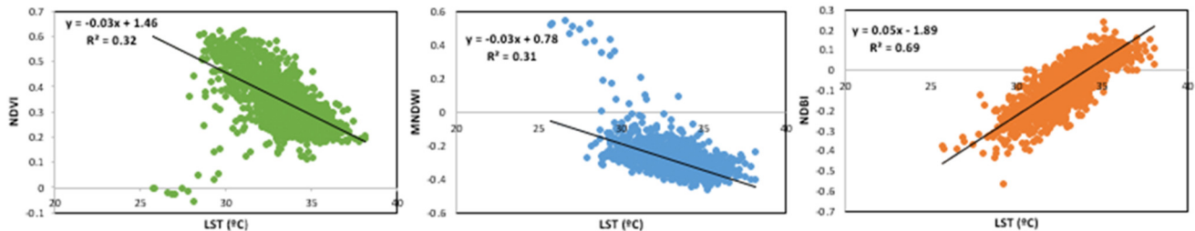
Figure 8. Correlation analysis between LST and landscape indices.
