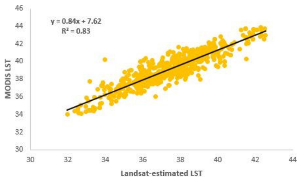
Figure 6. Correlation analysis between MODIS LST product and Landsat-estimated LST of 13 April 2023.
