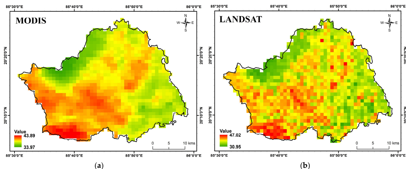
Figure 5. Spatial distribution of LST in Bhubaneswar: (a) MODIS LST product (MOD11A1); and (b) resampled Landsat-estimated LST.
