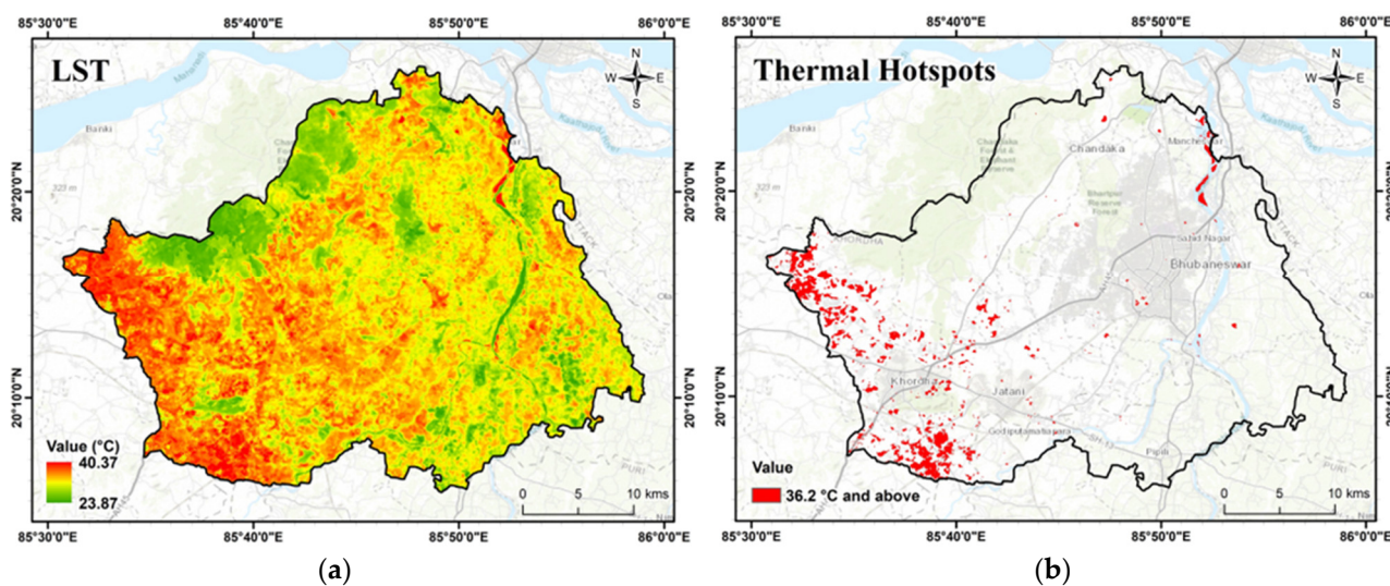
Figure 4. Spatial distribution of temperature in Bhubaneswar: (a) Land Surface Temperature (LST); and (b) thermal hotspots.
