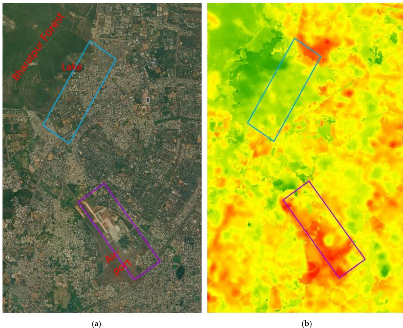
Figure 7. (a) Sample sites representative of neighbouring areas of blue-green spaces and non-blue-green spaces over the study area, and (b) LST visualisation of sample sites.
