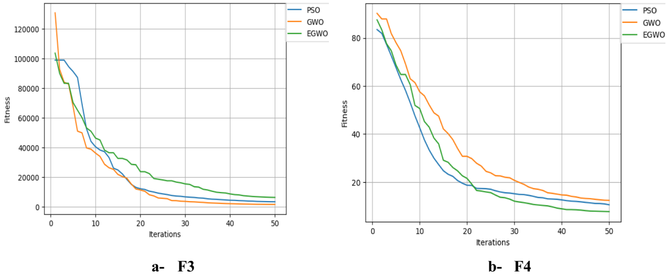
Fig. 11 Comparison of PSO [8], GWO [21], and A-GWO on Functions (F1, F4)
