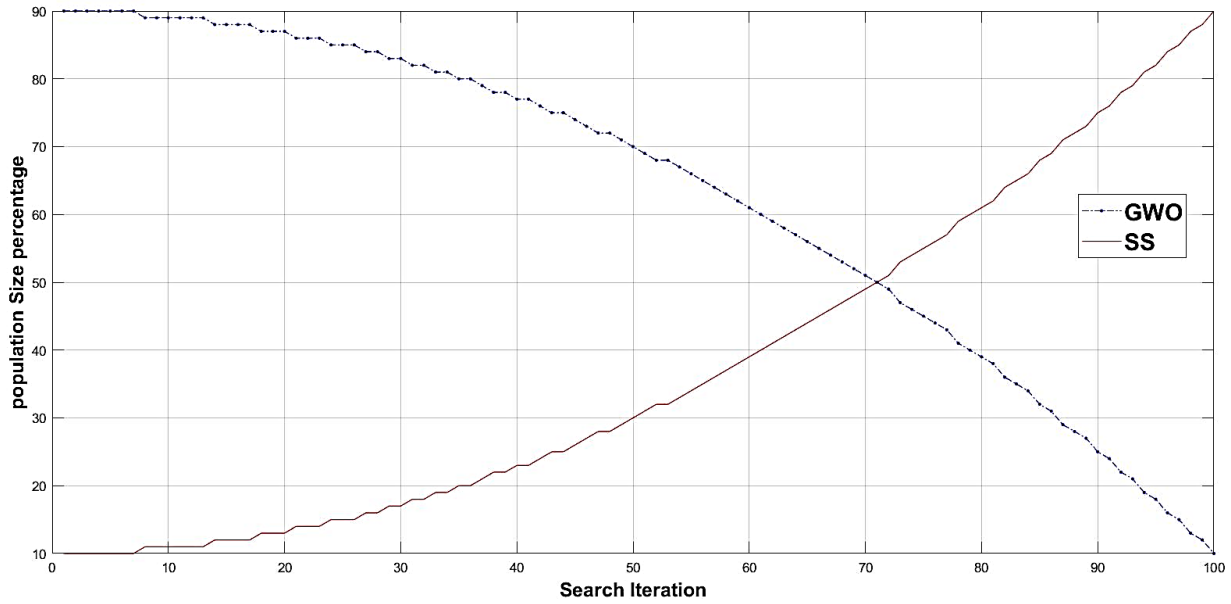
a- The first scenario (the proposed A-GWO senses stagnation in the search process)
