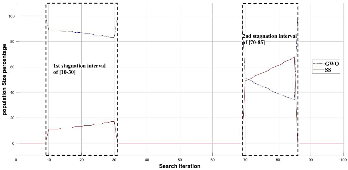
b- the second scenario (the proposed A-GWO stagnation during the [10-30] and [70-85])
