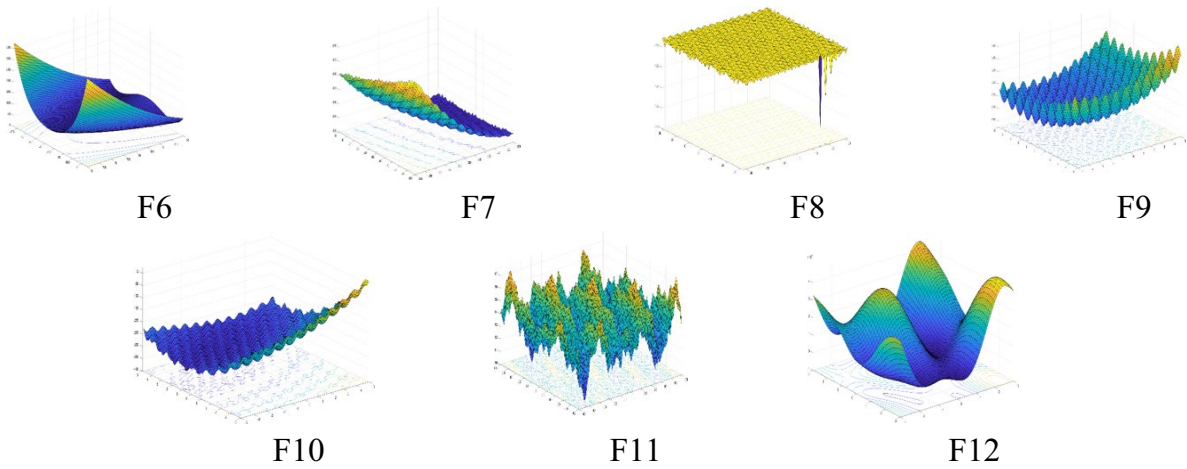
b- 2-D versions of multimodal benchmark functions (Basic Functions).
