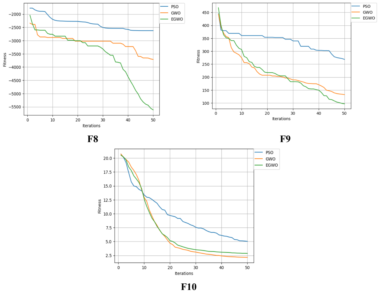
Fig. 12 Comparison of PSO [8], GWO [21], and A-GWO on Functions (F8, F9, and F10)
