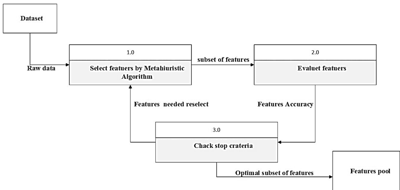
Fig. 2 Feature selection by wrapper model and optimization algorithm
