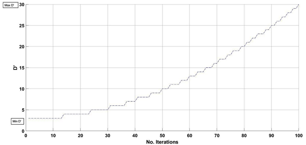
Fig. 9 Number of the updating dimensions in the 2nd group ( SS_g ) (where iter_{max}=100 , Max_{D_i}=30 , Max_{D_j}=3 )
