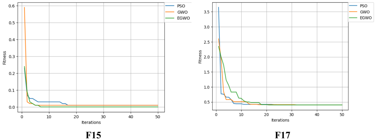
Fig. 14 Comparison of PSO [8], GWO [21], and A-GWO on Functions (F15, F17)
