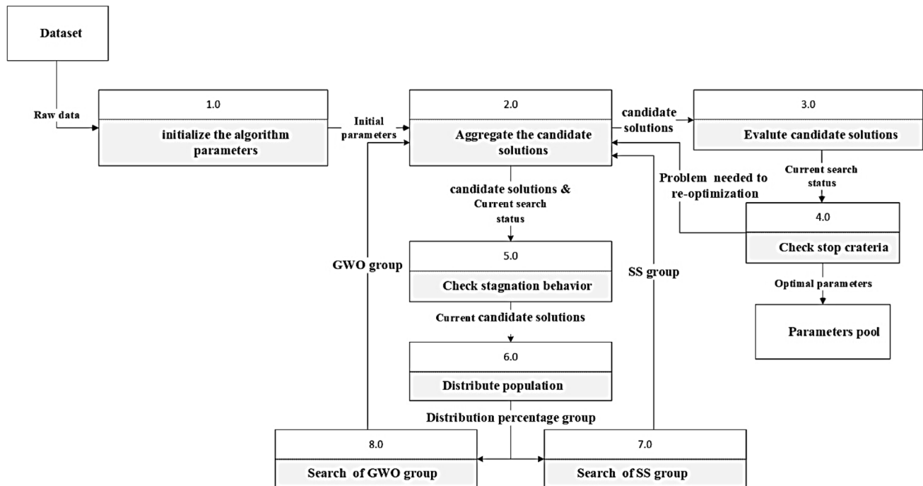
Fig. 7 Proposed a proactive grey wolf optimization (A-GWO)
