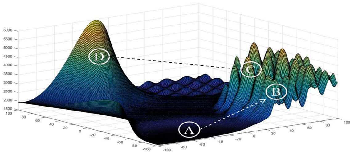
Fig. 6 Example of search processes of proposed A-GWO
