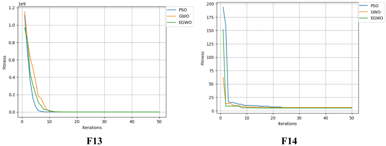
Fig. 13 Comparison of PSO [8], GWO [21], and A-GWO on Functions (F13, F14)
