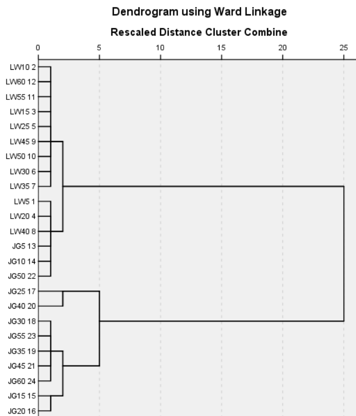
Figure 3: Dendrogram of hierarchical cluster analysis for the formulae LW and JG
