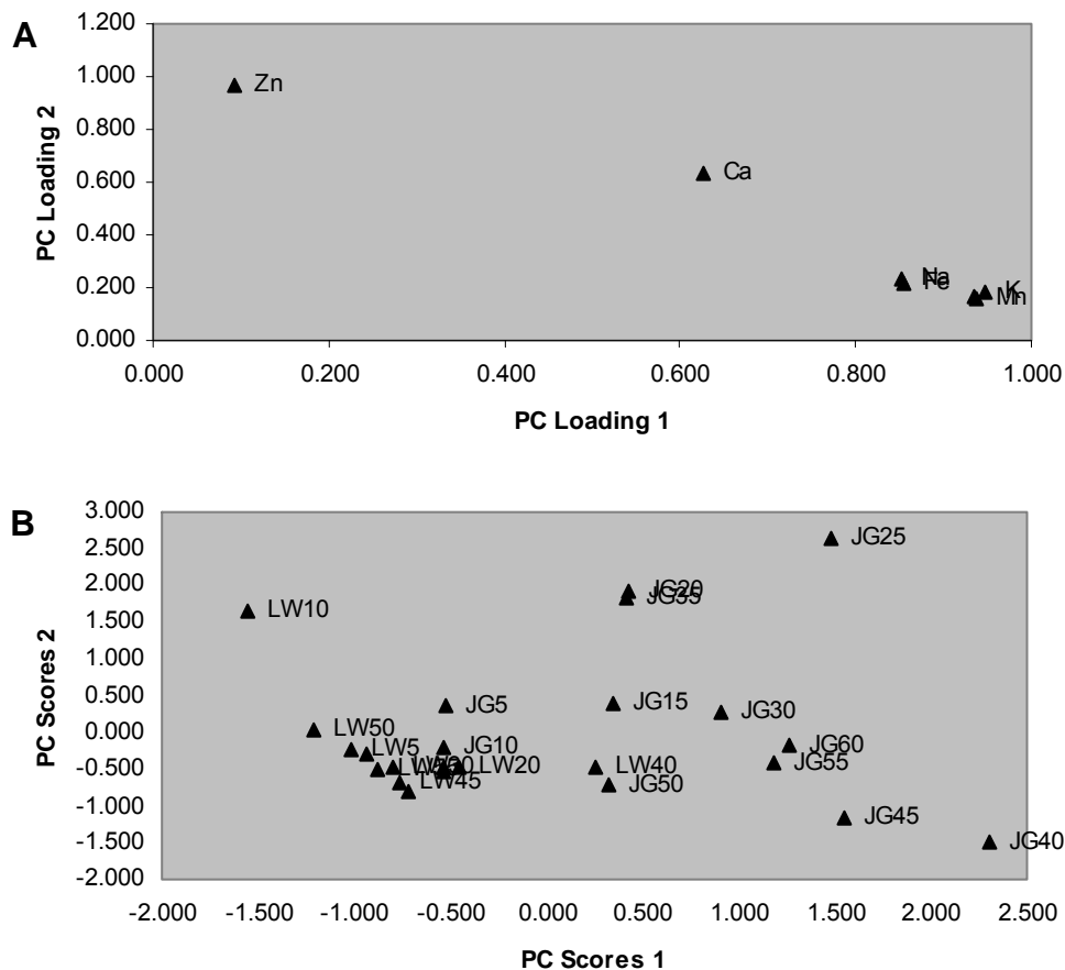
Figure 2: Varimax rotated principal component loadings (A) and scores (B), PC1 versus PC2
